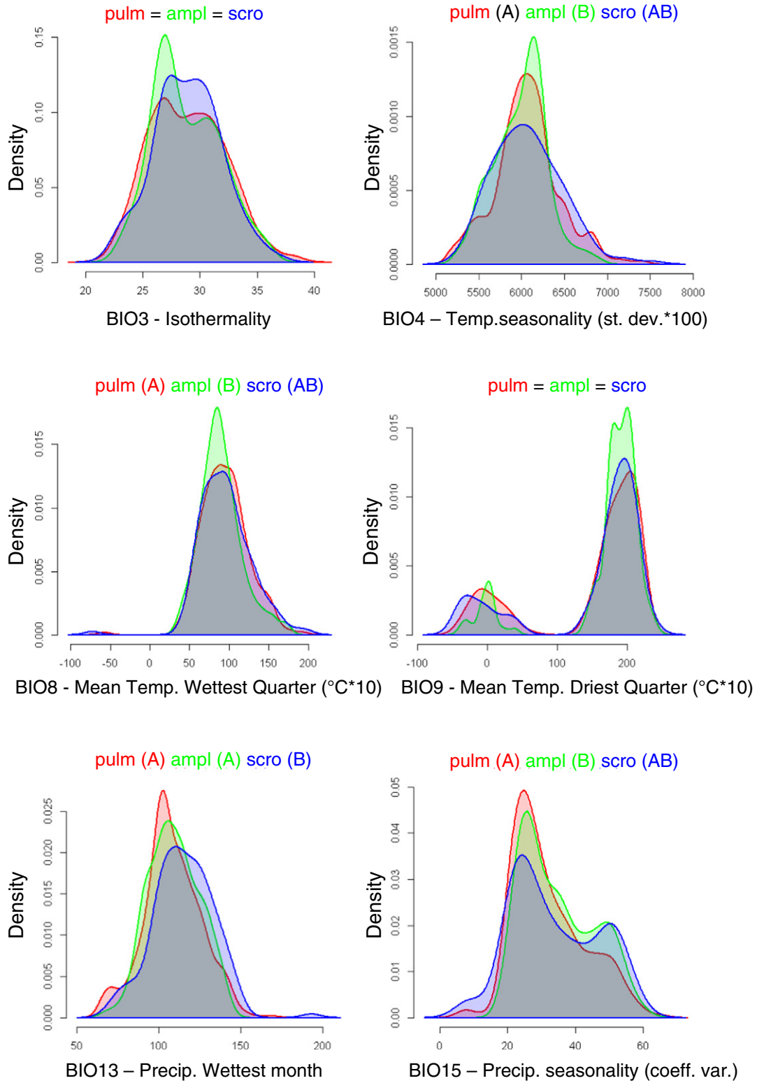
Fig. 2. Kernel density plots of the six climatic variables for the three species of Lobaria s. lat. in Italy. Differentiation among species and the results of Kruskal–Wallis tests are indicated in each plot. A lack of significant difference (at the P = 0.05 level) is indicated by an equal sign and same letter, while significant differences are indicated by either higher or lower signs and different letters. Pulm = Lobaria pulmonaria ; ampl = Lobaria amplissima ; scro = Lobaria scrobiculata .
