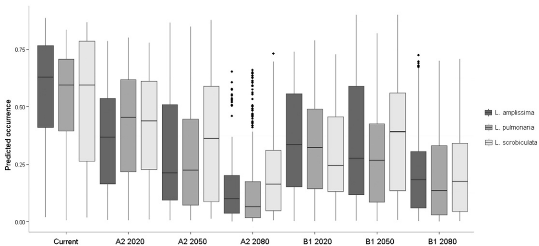
Fig. 5. Predicted occurrence of the three Lobaria s. lat. species in the 30 arc sec grid cells where the taxa have been actually observed in the current conditions. Predictions were carried out using two climate change scenarios (A2 and B1), for three time periods (2020, 2050 and 2080). The black line represents the median, black circle represents the mean, edge box corresponds to the first and third quartiles (the 25th and 75th percentiles), whiskers are 1.5 \cdot \text{IQR} (where IQR is the inter-quartile range).
