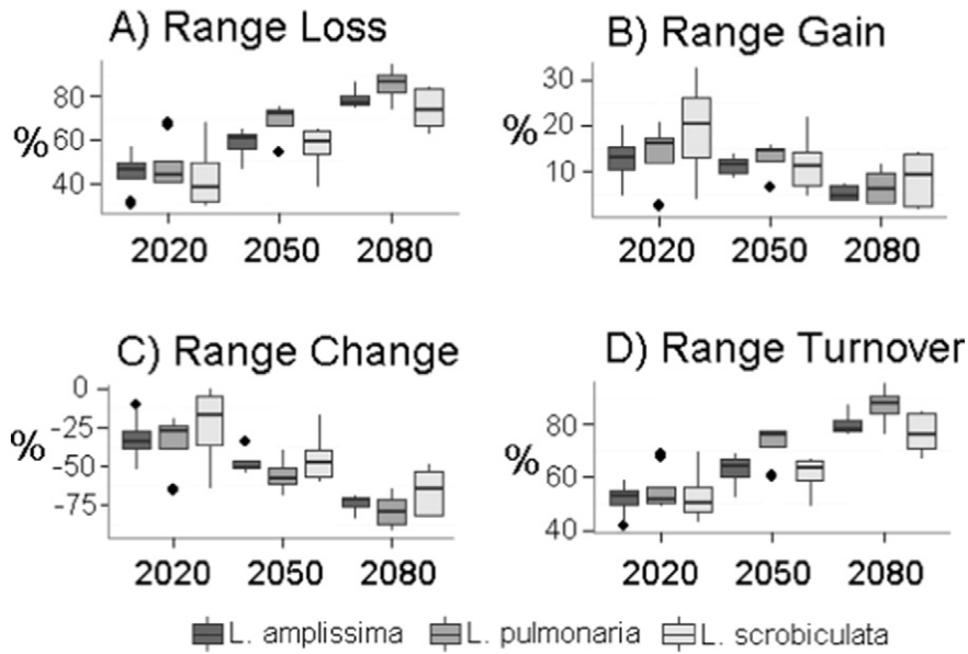
Fig. 4. Projected impacts of climate change on the distribution of the three species of Lobaria s. lat. in Italy as predicted using two climate change scenarios (A2 and B1), for three time periods (2020, 2050 and 2080). (A) Percentage of range loss (RL); (B) percentage of range gain (RG) and (C) percentage of range change (C); (D) percentage of range turnover (T). The black line represents the median, black circle represents the mean, edge box corresponds to the first and third quartiles (the 25th and 75th percentiles), whiskers are 1.5 \cdot \text{IQR} (where IQR is the inter-quartile range).
