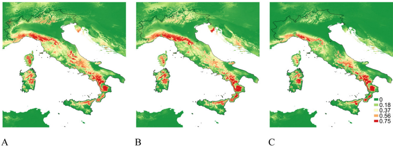
Fig. 3. Predicted habitat suitability in Italy for the three epiphytic Lobaria species, according to the Maxent models under current climatic conditions: A) Lobaria pulmonaria ; B) Lobarina scrobiculata ; C) Lobaria amplissima .
